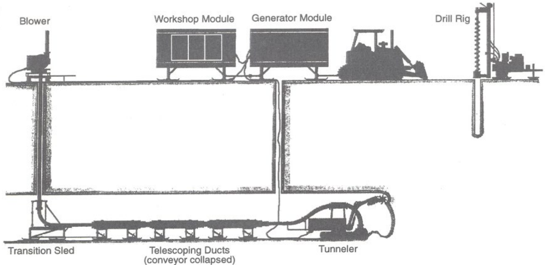
Figure 7. The South Pole Tunneling System (SPoTs).
